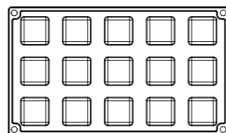
PX3220 Cube40time mm 34x34x34 h ~ 40 ml 15 impronte - indents
