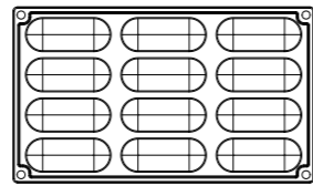
PX3216 Confy40time by Antonio Bachour mm 80x30x24 h ~ 40 ml 12 impronte - indents
