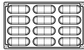
PX3215 Pastel40time by Antonio Bachour mm 80x27x21 h ~ 40 ml 12 impronte - indents
